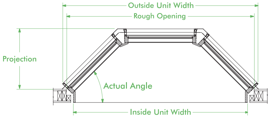
45° Angle Bay 1-5 Flankers with 1-5 Center
