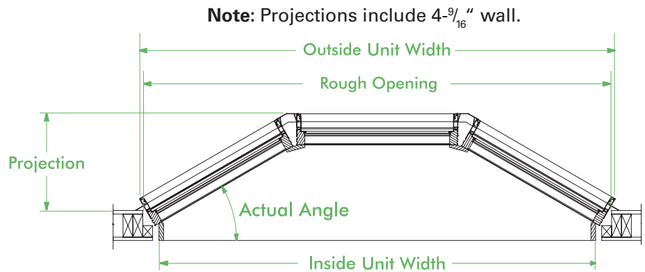
30° Angle Bay 1-5 Flankers with 1-5 Center
